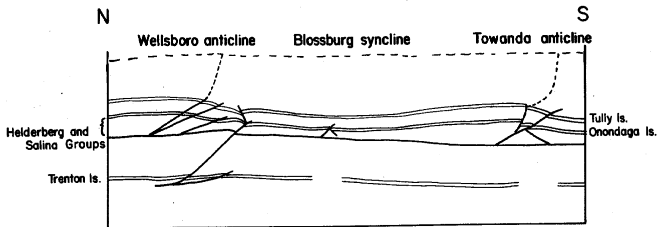
Figure 9. Seismic section (interpreted from proprietary data) of a part of the Allegheny plateau in Pennsylvania. Note the thickening of the beds of the Helderberg and Salina Groups in the cores of the anticlines. Uplimb thrusts from the tepee structures.
