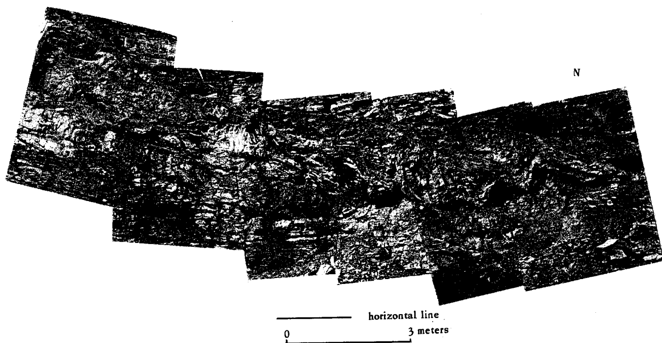
Figure 13. Photomosaic of the Bridge Street fault. Lower beds are horizontal.
