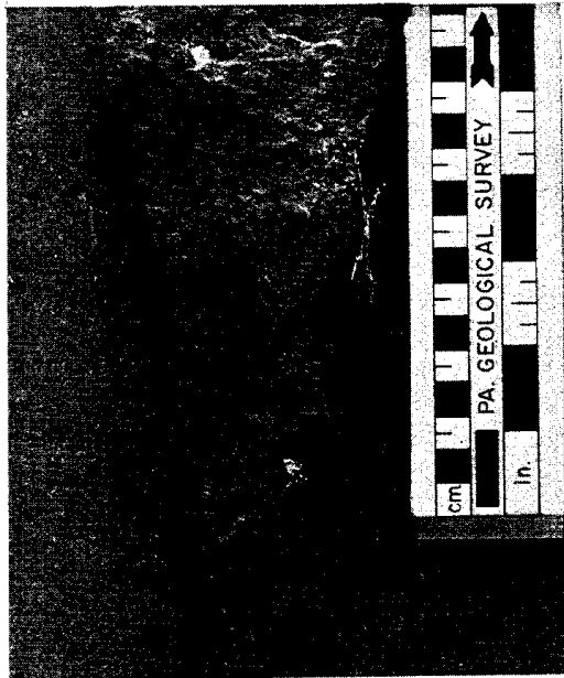
B. Close-up of Cruziana showing endopodite markings; from below 20 m, Figure 28.
