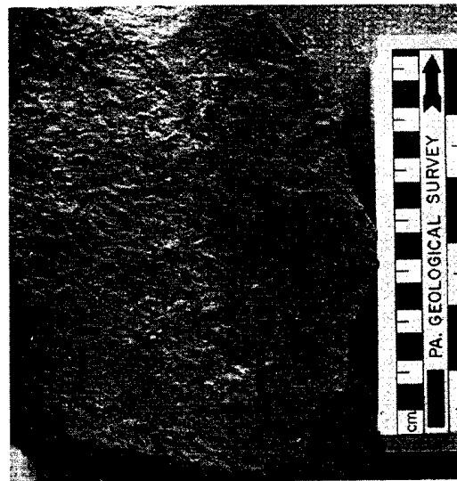
E. Abundant small ? planolites from below 20 m, Figure 28.
