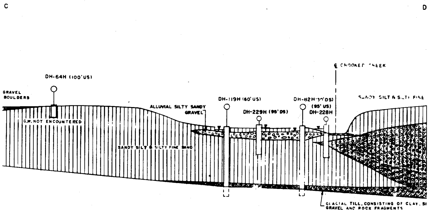
Figure 24. Soil Profile Along Axis of Hammond Dam.
