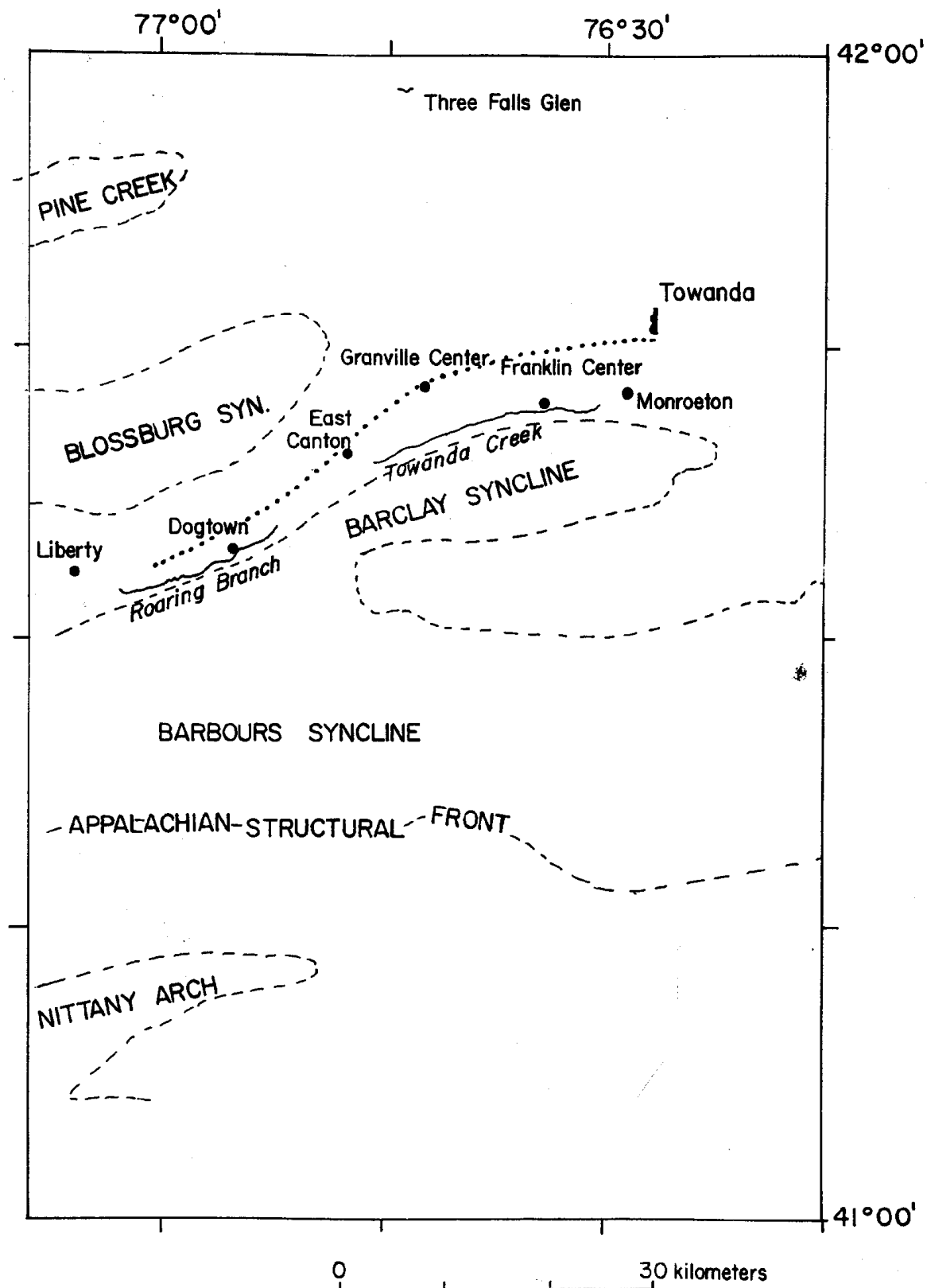
Figure 14. Index map, showing place names used in the text. Dashed lines indicate topographic expression of synclines and the Nittany arch. Dotted line represents probable surface trace of Bridge Street fault.
