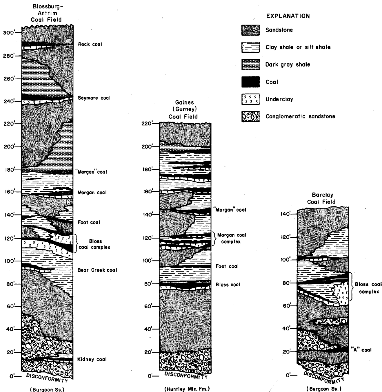
Figure 7. Generalized Pennsylvanian stratigraphic columns of the Blossburg-Antrim, Gaines, and Barclay coal fields.
