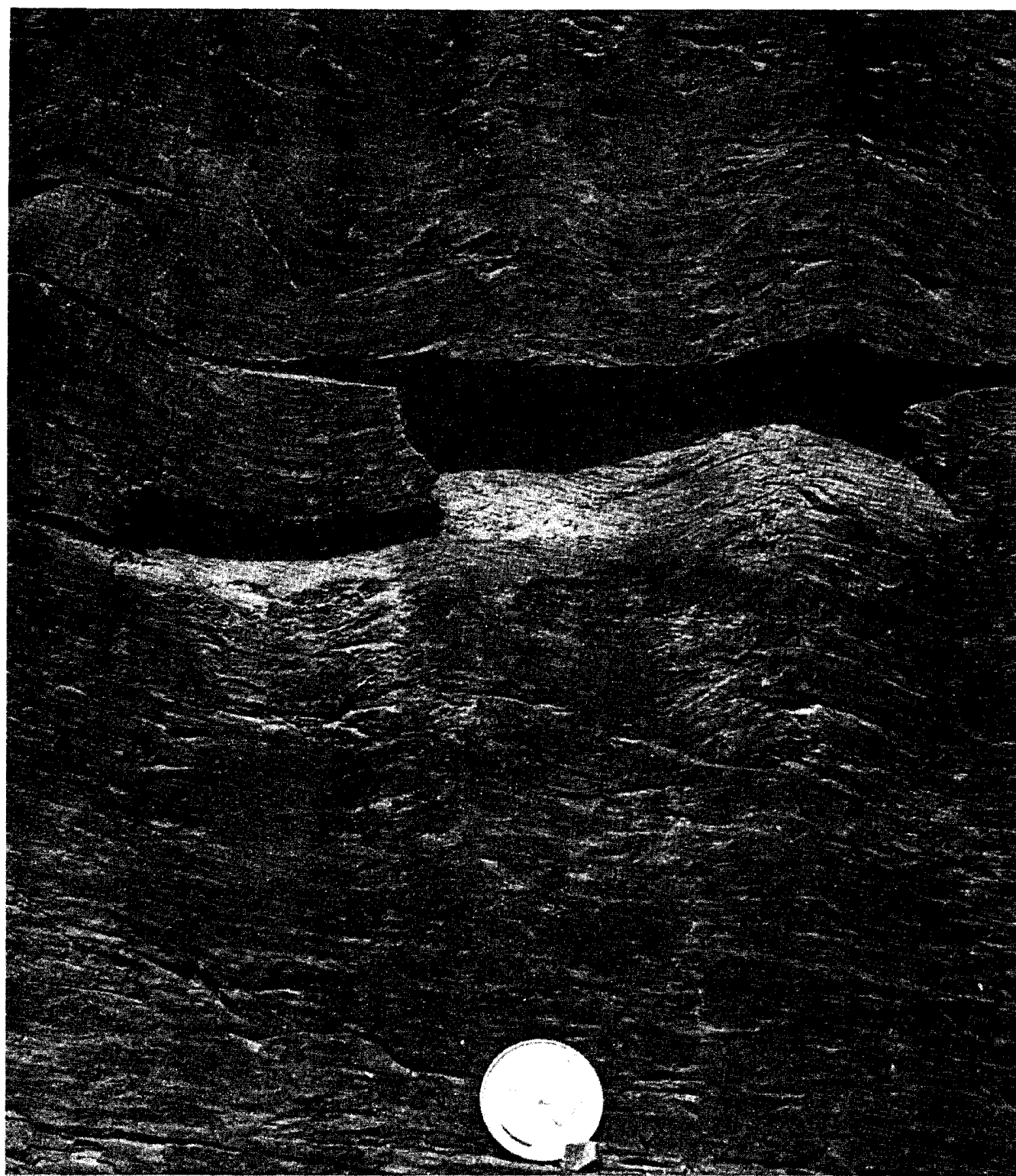
Sinusoidal overprinting and minute uplimb thrusts on flat-lying beds.
