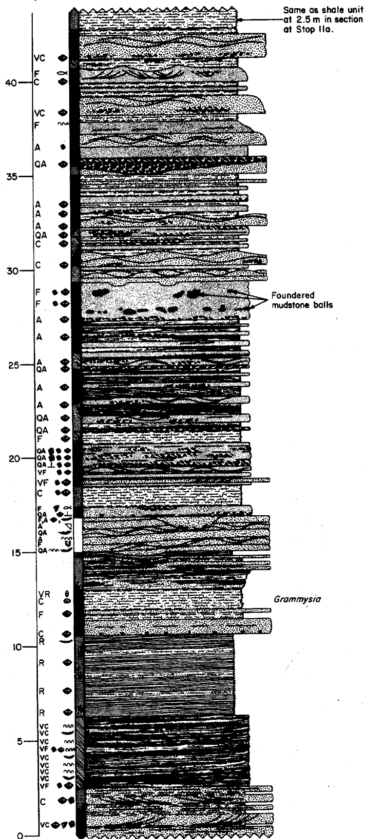
FIGURE 36. COLUMNAR SECTION SHOWING MARINE SUCCESSION IN LOCK HAVEN FORMATION AT STOP 11b. KEY IS ON FACING PAGE.
