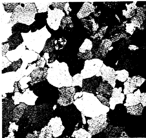
A. Pottsville quartzarenite; x28; crossed nicols.
