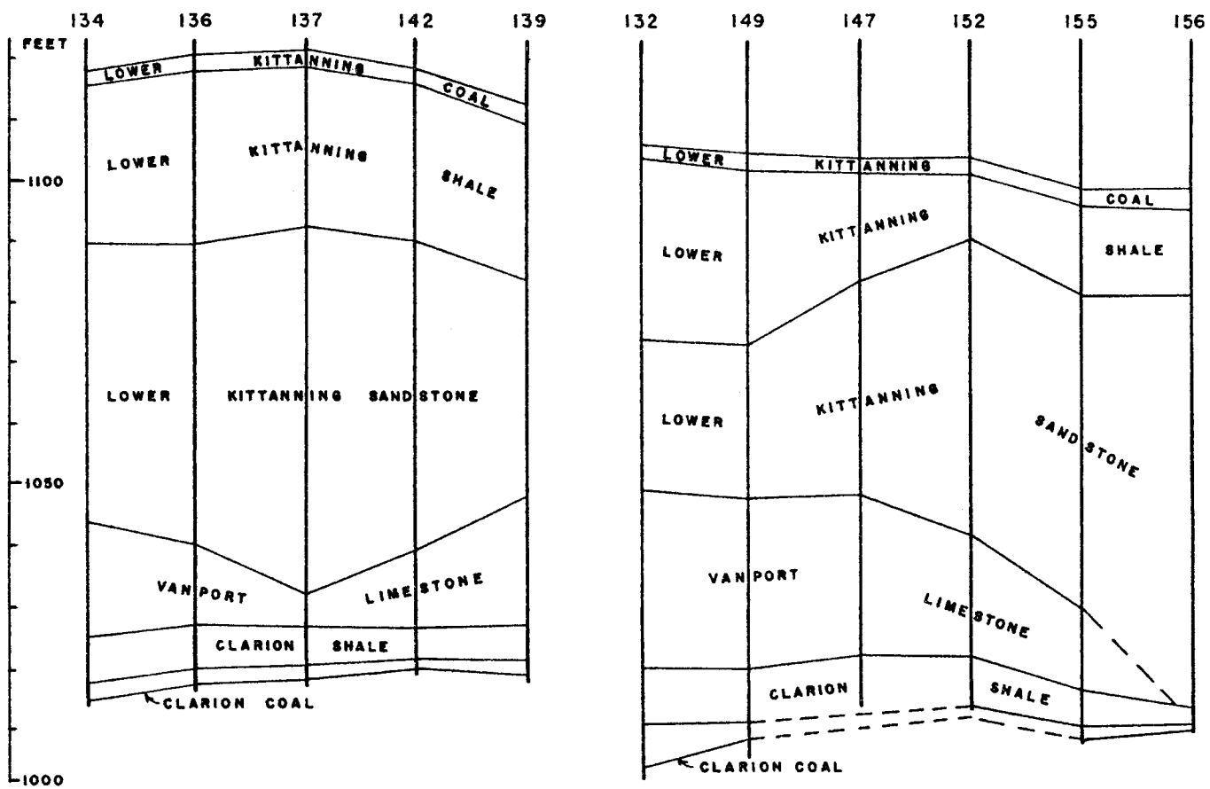
Cross-Sections of Vanport Limestone Mine Penn-Dixie Cement Corp., West Winfield, Pa. (See map for bore hole locations)
